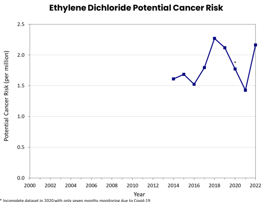
Figure 33: Ethylene Dichloride Annual Average Potential Cancer Risk at Beacon Hill, 2014–2022
