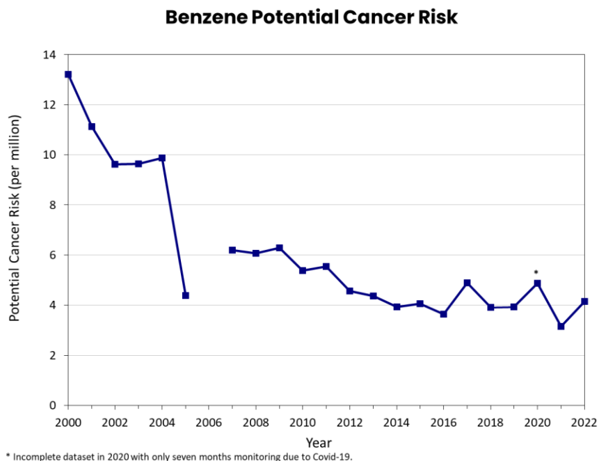
Figure 28: Benzene Annual Average Potential Cancer Risk at Beacon Hill, 2000–2022
