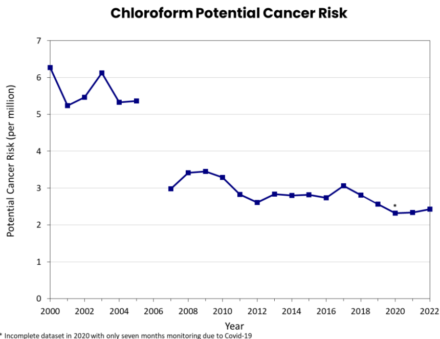
Figure 32: Chloroform Annual Average Potential Cancer Risk at Beacon Hill, 2000–2022
