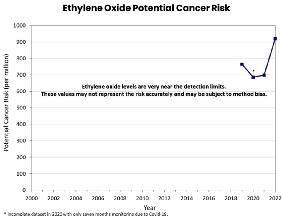
Figure 25: Ethylene Oxide Annual Average Potential Cancer Risk at Beacon Hill, 2019–2022
