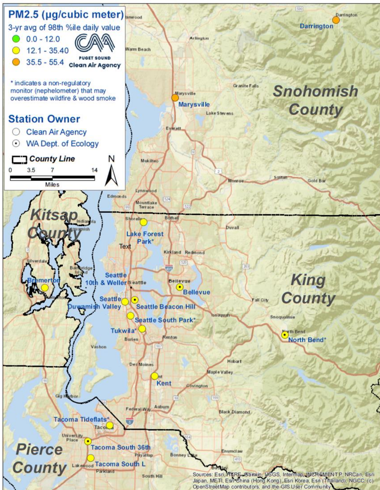
Map 2: The 98th Percentile 3-Year Average Daily PM 2.5 Concentrations for 2022
