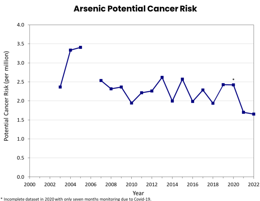
Figure 29: Arsenic Annual Average Potential Cancer Risk at Beacon Hill, 2003–2022
