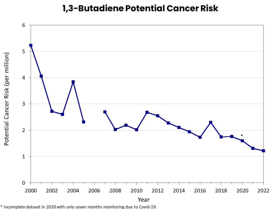
Figure 34: 1,3-Butadiene Annual Average Potential Cancer Risk at Beacon Hill, 2000–2022
