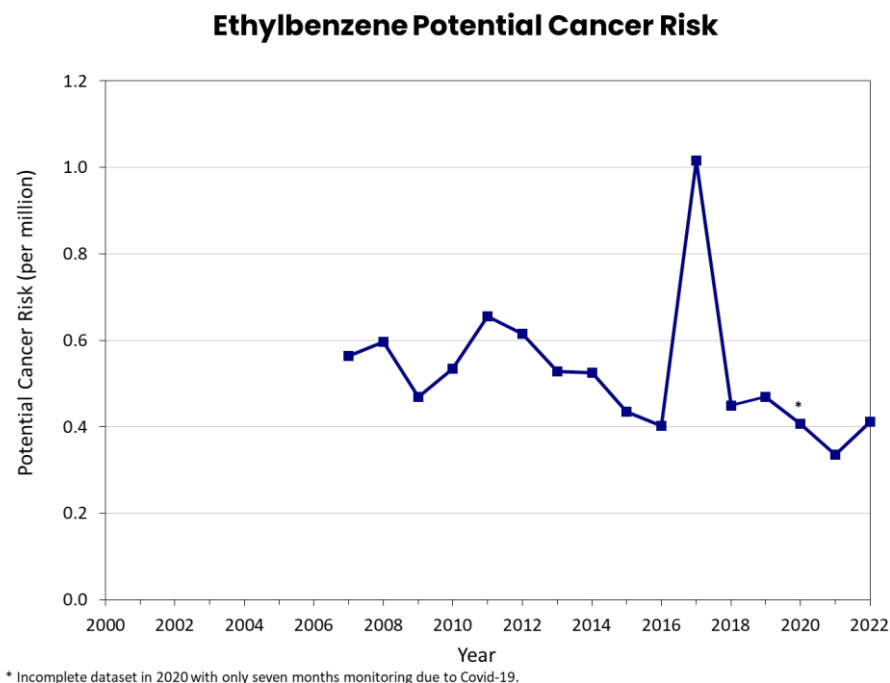
Figure 37: Ethylbenzene Annual Average Potential Cancer Risk at Beacon Hill, 2007–2022
