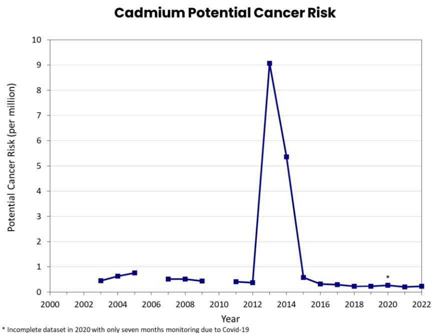
Figure 38: Cadmium Annual Average Potential Cancer Risk at Beacon Hill, 2003–2022
