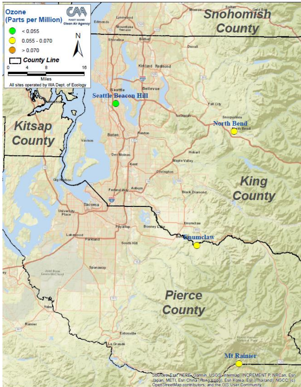
Map 3: Ozone 3-year Average of 4th Highest 8-hr Value for 2022
