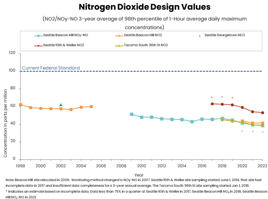
Figure 21: Nitrogen Dioxide (NO 2 ) (1998–2005; 2017–2022) and Reactive Nitrogen (NO y – NO) (2007–2022) for the Puget Sound Region
