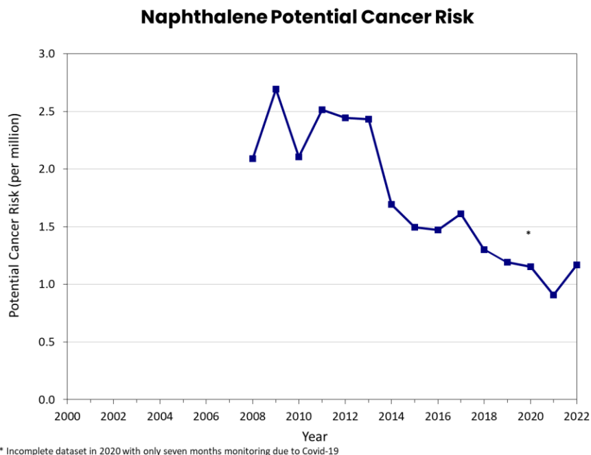
Figure 35: Naphthalene Annual Average Potential Cancer Risk at Beacon Hill, 2008–2022
