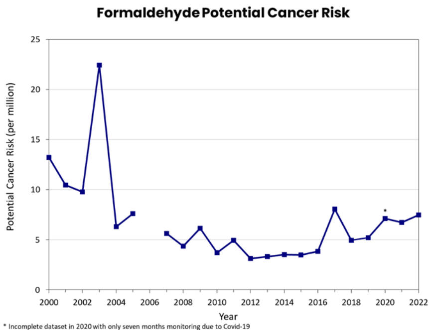
Figure 26: Formaldehyde Annual Average Potential Cancer Risk at Beacon Hill, 2000–2022
