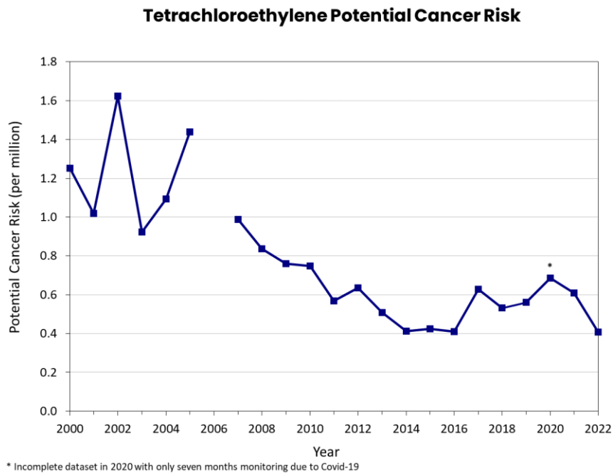
Figure 36: Tetrachloroethylene Annual Average Potential Cancer Risk at Beacon Hill, 2000–2022
