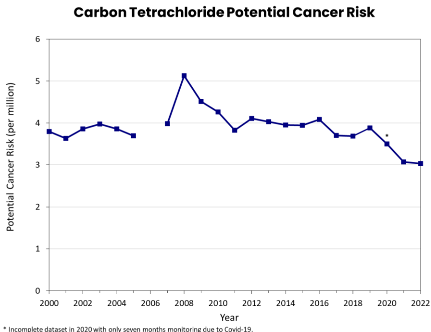
Figure 31: Carbon Tetrachloride Annual Average Potential Cancer Risk at Beacon Hill, 2000–2022
