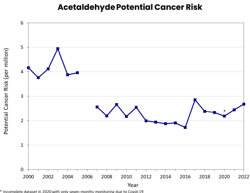
Figure 30: Acetaldehyde Annual Average Potential Cancer Risk at Beacon Hill, 2000–2022
