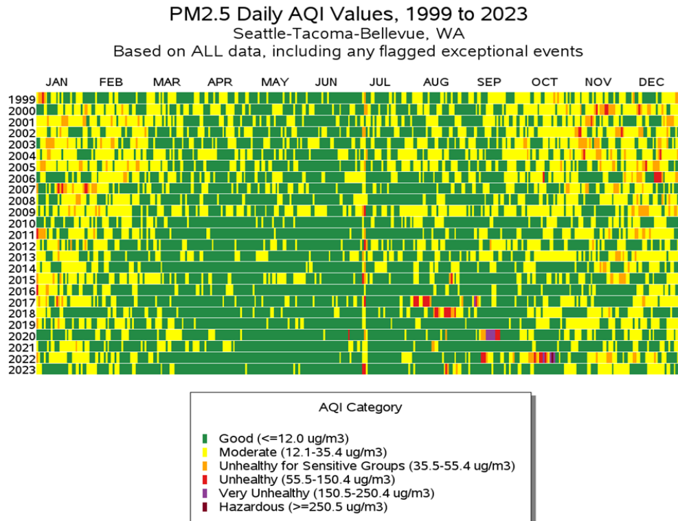
Figure 1: PM 2.5 Daily AQI Values for Seattle-Tacoma-Bellevue, WA from 1999–2023.
