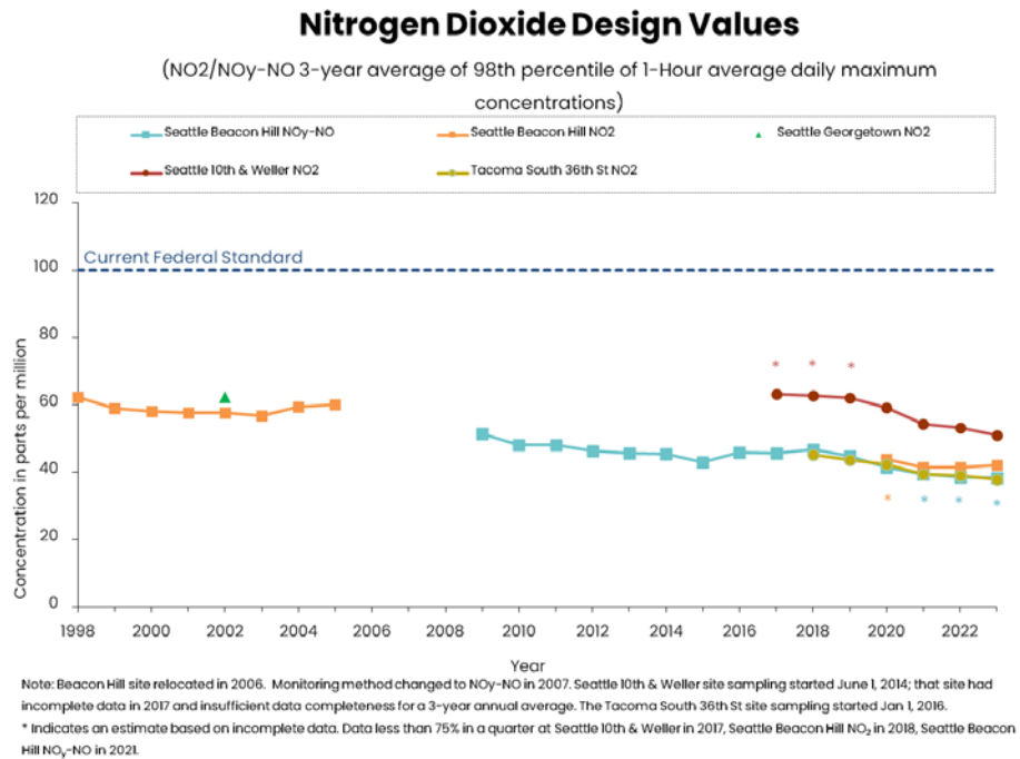
Figure 21: Nitrogen Dioxide (NO 2 ) (1998–2005; 2017–2023) and Reactive Nitrogen (NO y – NO) (2007–2023) for the Puget Sound Region
