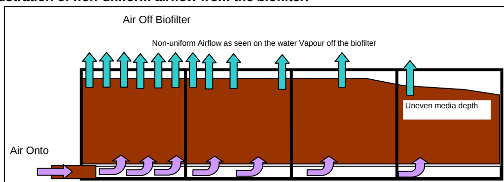
Figure 3: Illustration of non-uniform airflow from the biofilter.
