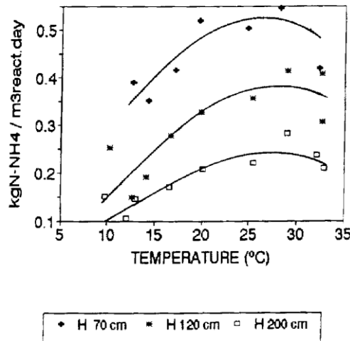
Figure 3. Ammonium oxidation rate (kg N/m 3 d) versus temperature. The symbols represent three different heights in a biofilter (Fdz-Polanco et al. , 1994).
